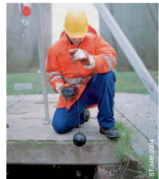
Dräger CMS with Remote-System: Measurement with extension hoses of up to 10 m in length.
